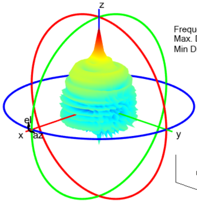
helixMultifilar
