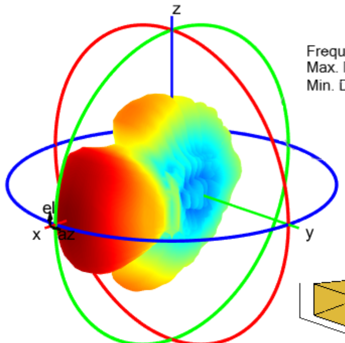
helixMultifilar
